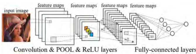
Fig. 2: Inference (aka feedforward) phase in CNN
