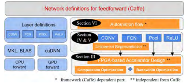
Fig. 1: Overview of Caffeine Framework
