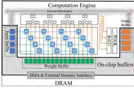
Figure 5: Scalable accelerator architecture design
