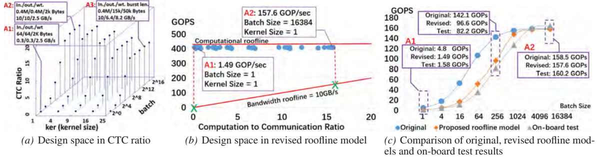
Figure 8: Design space exploration for FCN input-major mapping under various batch and kernel sizes
