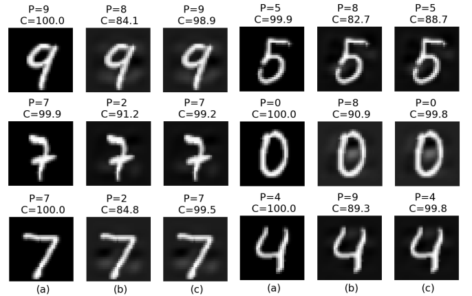
Fig. 2: Comparison of prediction ( P=. ) class with the highest confidence ( C=..% ) by the protected LeNet-3 on MNIST dataset: (a) clean inputs, our attack; (b) crafted inputs, our attack; (c) crafted inputs, no (hardware parameter) attack.
