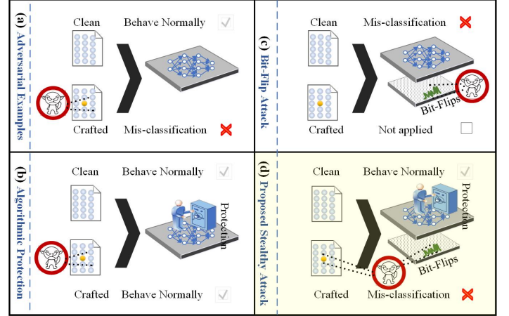
Fig. 1: Our “stealthy” attack against a protected DNN via smart bit flipping of DNN weights. Both the DNN inputs and parameters are perturbed. The DNN works correctly for clean inputs, but misclassifies inconspicuous crafted inputs.
